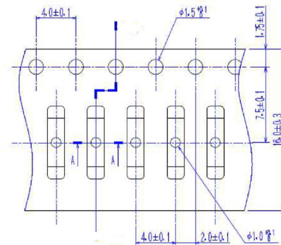
New Spec, 4 mm Pitch
