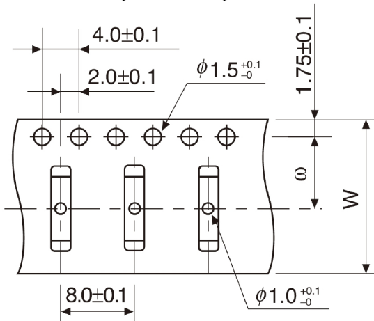
Old Spec, 8 mm Pitch
